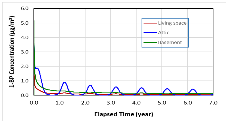
Figure 2-18. Predicted Gas-Phase 1-BP Concentrations ( \text{Mg}/\text{M}^3 ) in Three Locations Within the Attic/Living Space/Crawlspace Building Configuration.
