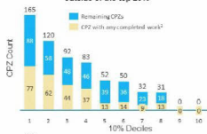
% of top decile of risk (Dx model) that moves outside of the top 20%
